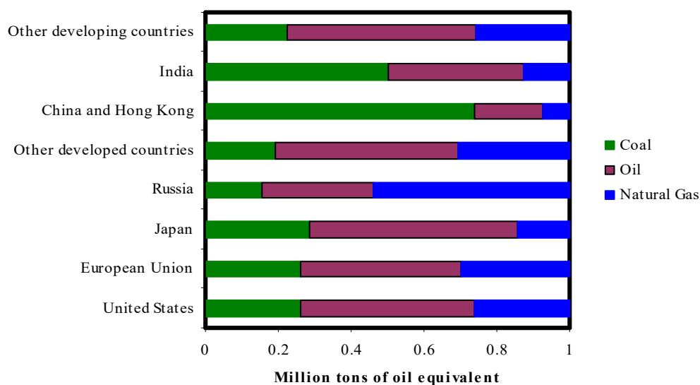
Figure 9. Conventional energies
