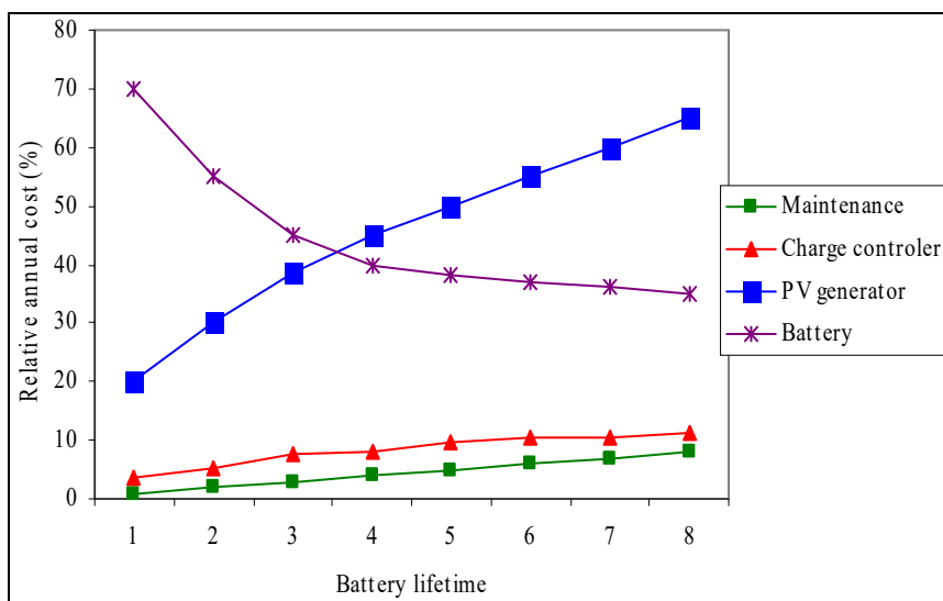
Figure 12. Battery lifetime versus relative annual cost (%)
