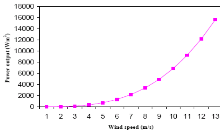
Wind speed vs Power output
