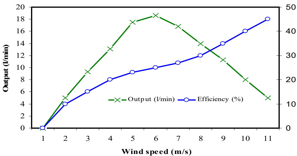
Figure 6. Wind pumps output and efficiency
