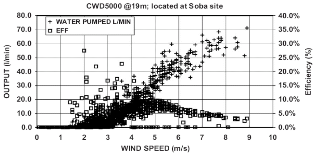
Figure 4. Performance of the CWD 5000
