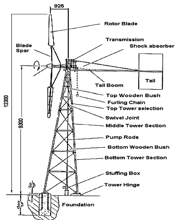
Figure 3. Schematic of the construction of the wind pump
