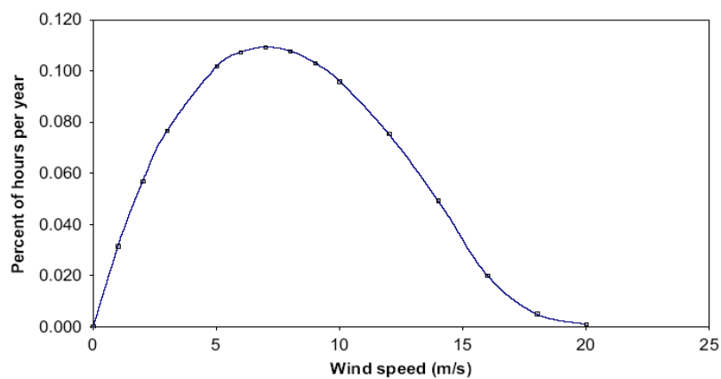
Figure 2. Yearly wind probability density ( k = 1.99, c = 7.81\text{ms}^{-1} )
