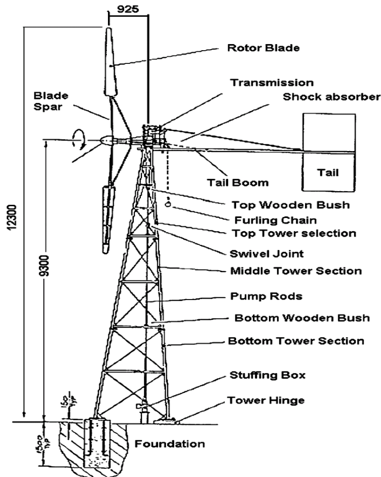
Figure 3. Schematic of the construction of the wind pump
