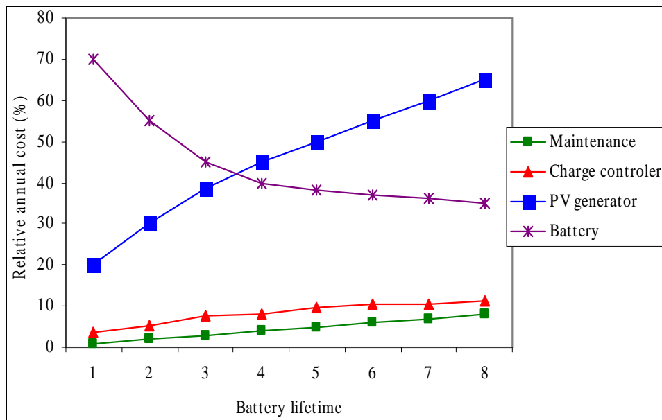
Figure 12. Battery lifetime versus relative annual cost (%)
