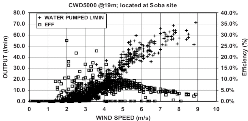
Figure 4. Performance of the CWD 5000
